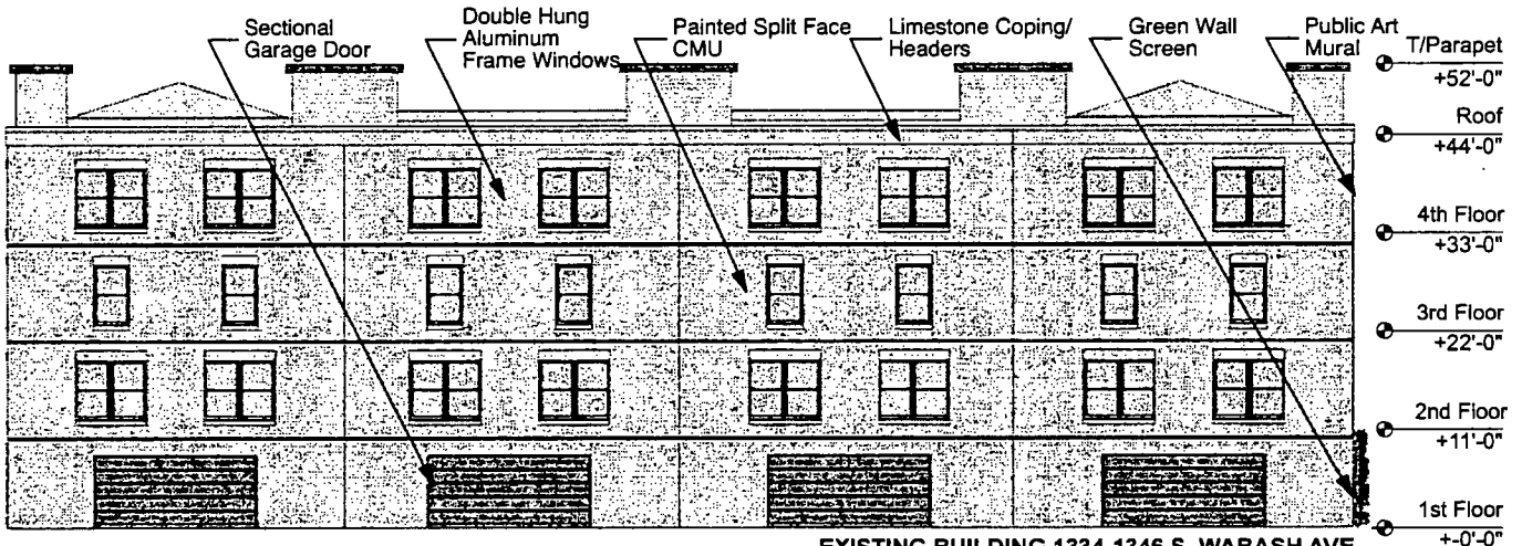
EXISTING BUILDING 1334-1346 S. WABASH AVE. WEST ELEVATION
