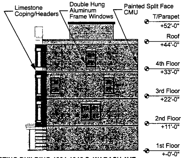
EXISTING BUILDING 1334-1346 S. WABASH AVE. NORTH ELEVATION
