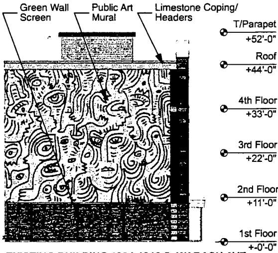
EXISTING BUILDING 1334-1346 S. WABASH AVE. SOUTH ELEVATION
