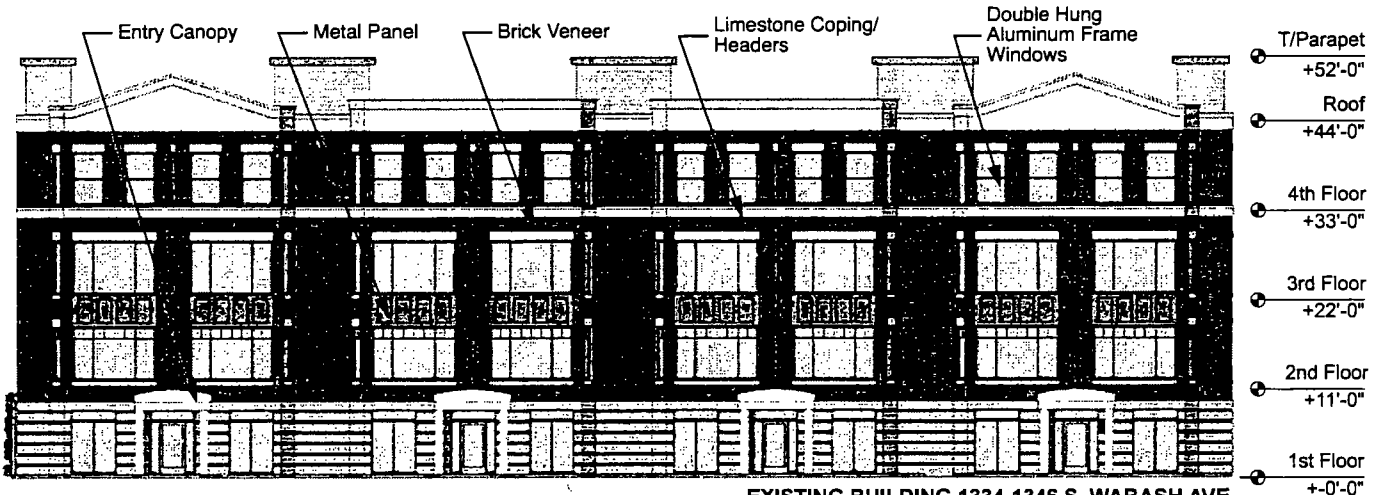
EXISTING BUILDING 1334-1346 S. WABASH AVE. EAST ELEVATION
