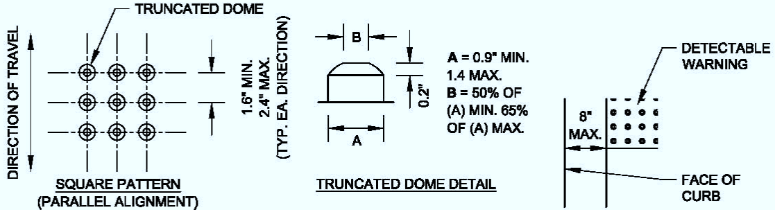
UNIT PATTERN & DOME DETAIL
